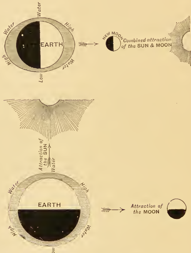
FIG. 114.—Spring and neap tides.
